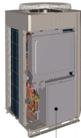
Compressor compartment
